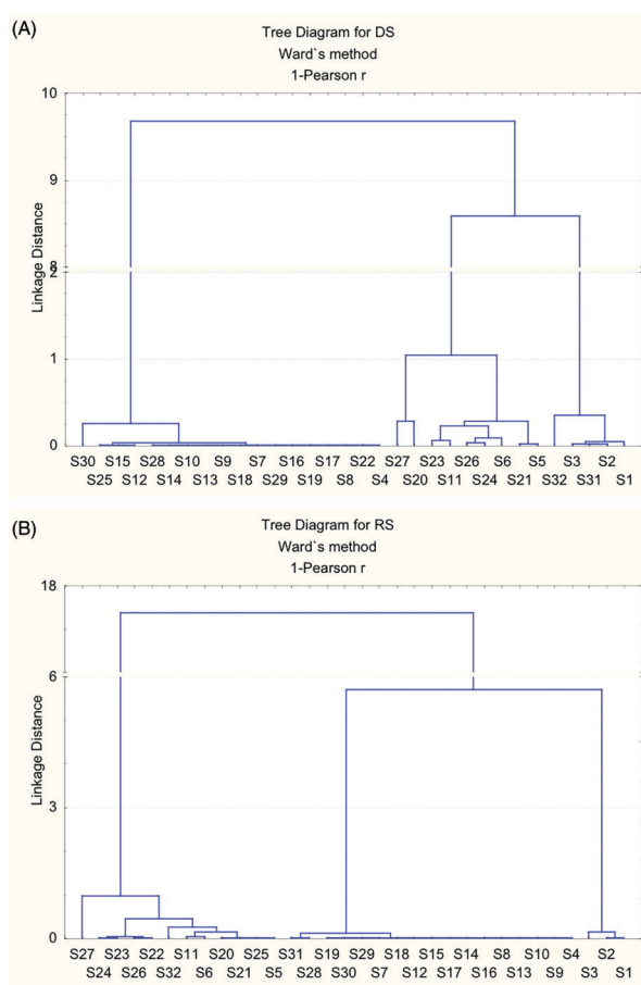
Figure 7. Cluster analysis: (A) dry season (DS) and (B) rainy season (RS) at the Ring of Cenotes (RC).
